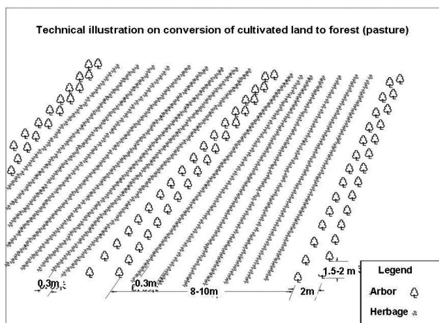
Figure 1. Two-row belt scheme with row/plant spacing of 2m and belt spacing of 8m. Trees species include Populus popularis and Populus alba var. pyramidalis , inter-cropping forage/fodder is Medicago sativa . Drawing by: GUO Huimei, Inner Mongolia Forestry Survey and Planning Institute
