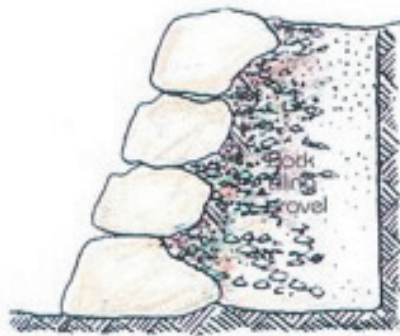
Stone constructed soil retaining works
