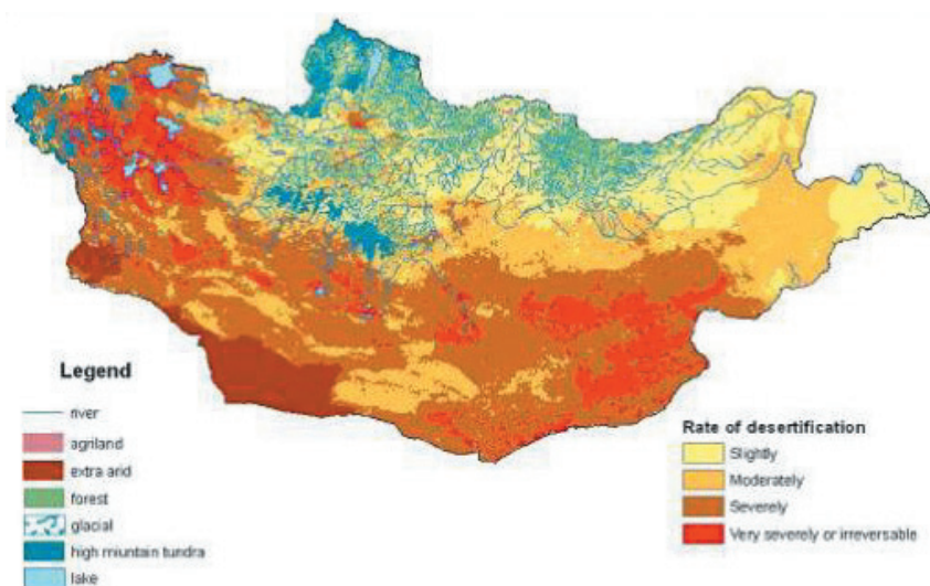
Figure 1. Extent and location of desertification in Mongolia in 2006
