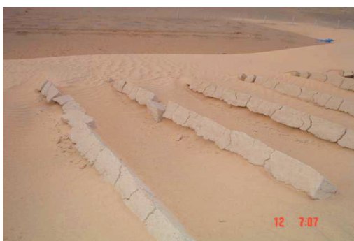
Figure 9 and 10. Clay barrier and Net checkerboard
