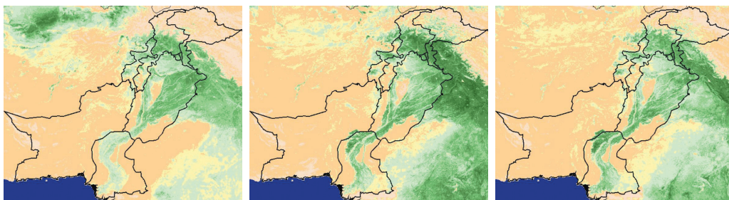
Figure 1. Mean monthly NDVI for the months of April (spring), August (monsoon), and October (autumn)
